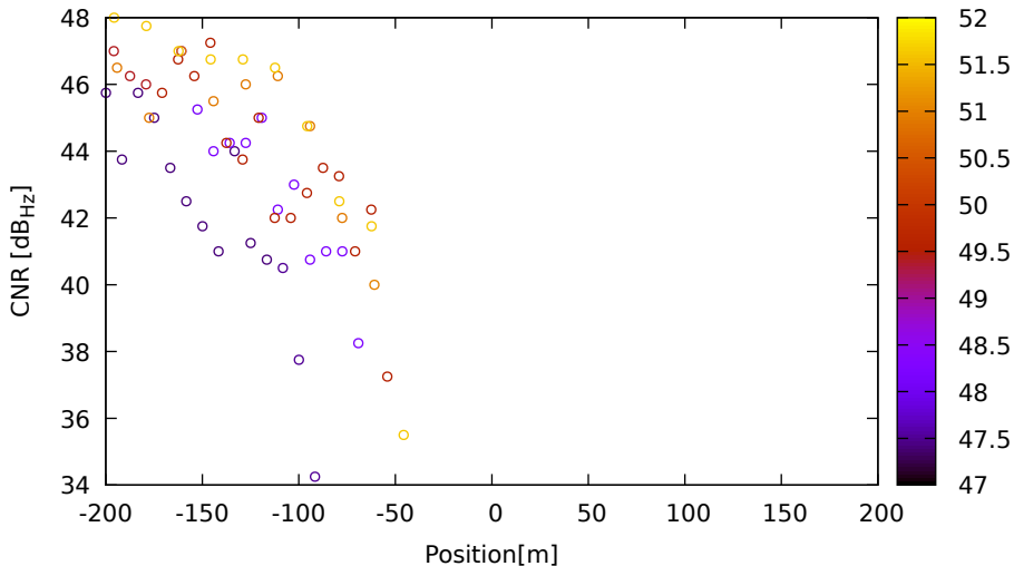
CNR vs position for E34 (E5a) on LeicaGS15 - DOY 262 jam. 1
