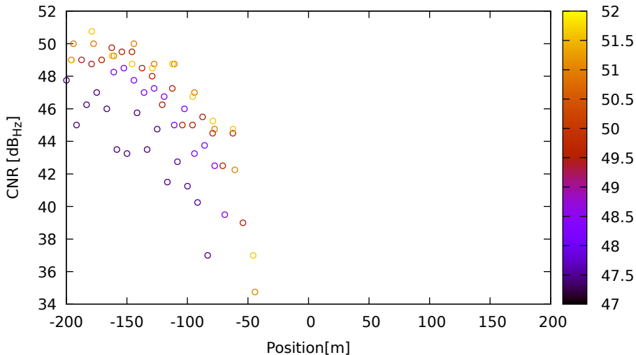
CNR vs position for E34 (E5b) on LeicaGS15 - DOY 262 jam. 1
