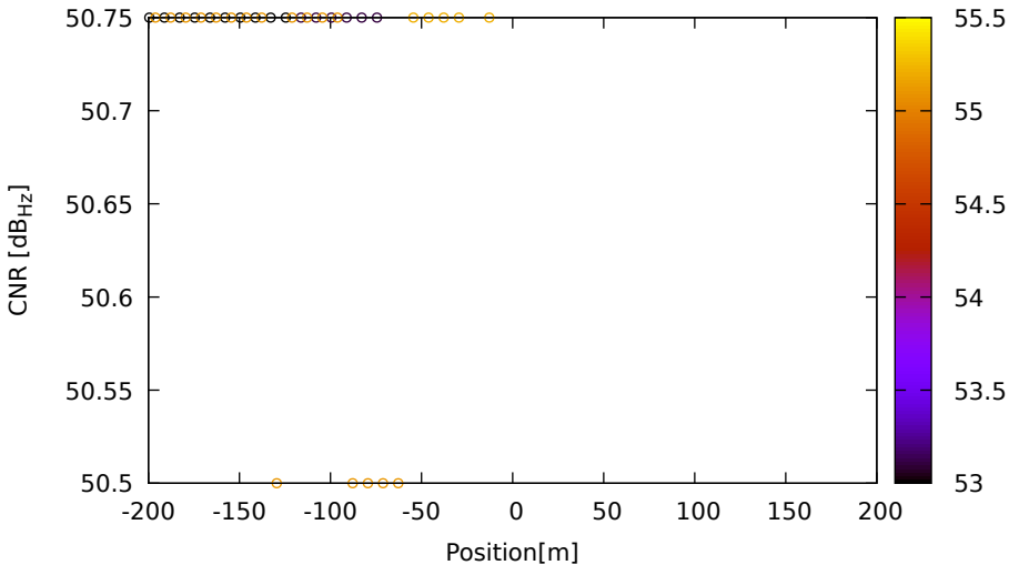
CNR vs position for E34 (E5b) on LeicaGS15 - DOY 262 jam. 2
