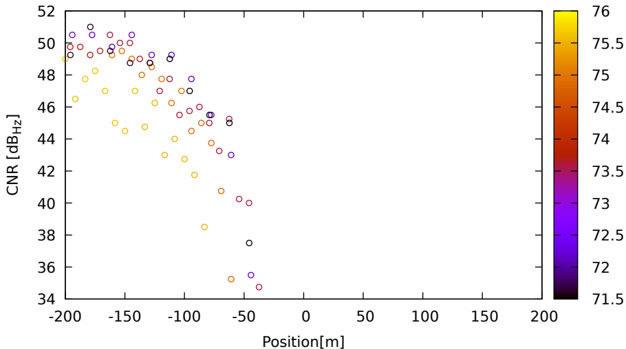
CNR vs position for E36 (E5b) on LeicaGS15 - DOY 262 jam. 1
