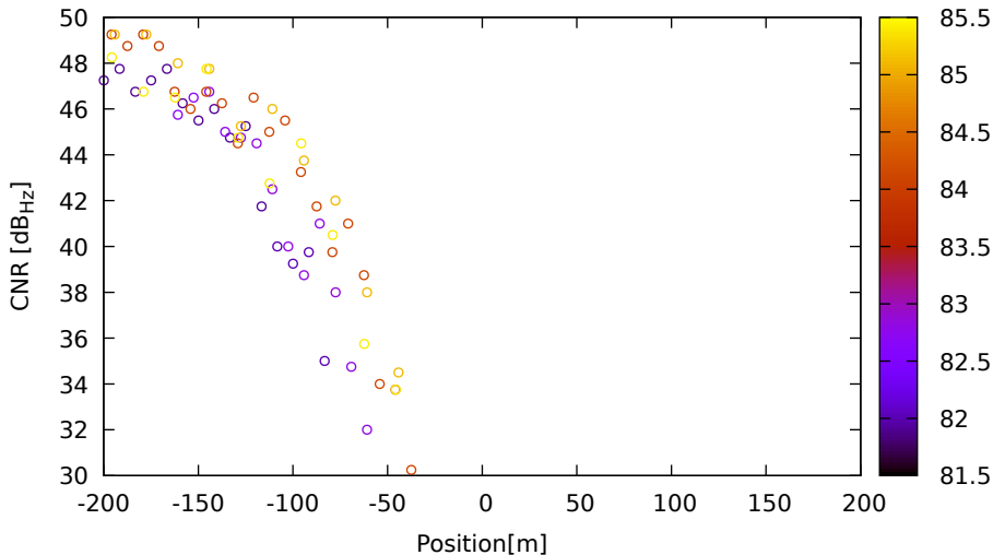
CNR vs position for G01 (L1) on LeicaGS15 - DOY 262 jam. 1
