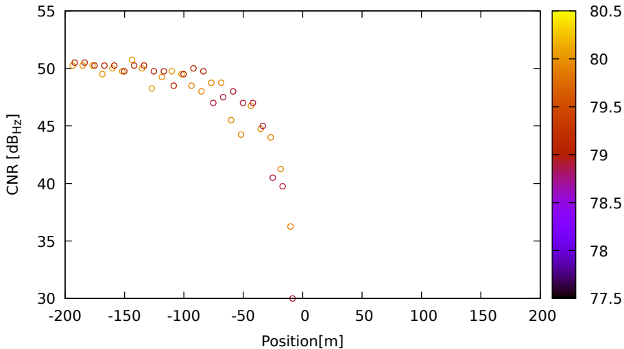
CNR vs position for G01 (L1) on LeicaGS15 - DOY 262 jam. 3
