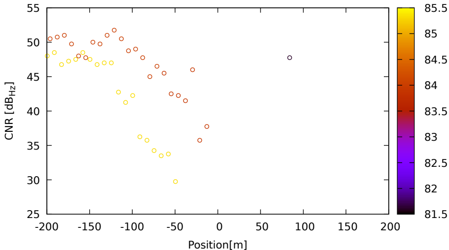
CNR vs position for G01 (L2) on LeicaGS15 - DOY 262 jam. 2
