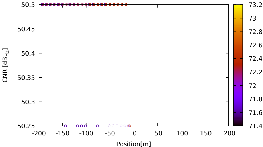
CNR vs position for G03 (L5) on LeicaGS15 - DOY 262 jam. 3
