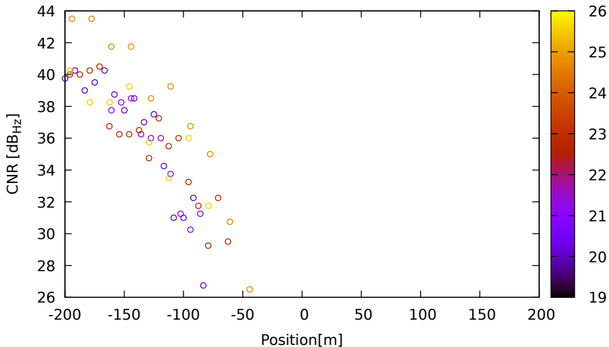
CNR vs position for G04 (L1) on LeicaGS15 - DOY 262 jam. 1
