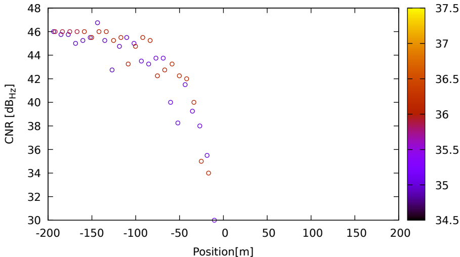
CNR vs position for G04 (L1) on LeicaGS15 - DOY 262 jam. 3
