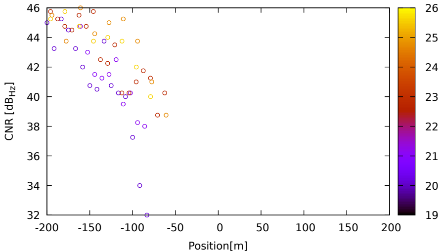
CNR vs position for G04 (L5) on LeicaGS15 - DOY 262 jam. 1
