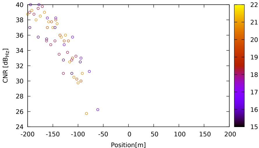
CNR vs position for G08 (L1) on LeicaGS15 - DOY 262 jam. 1
