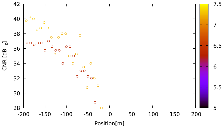
CNR vs position for G08 (L1) on LeicaGS15 - DOY 262 jam. 3
