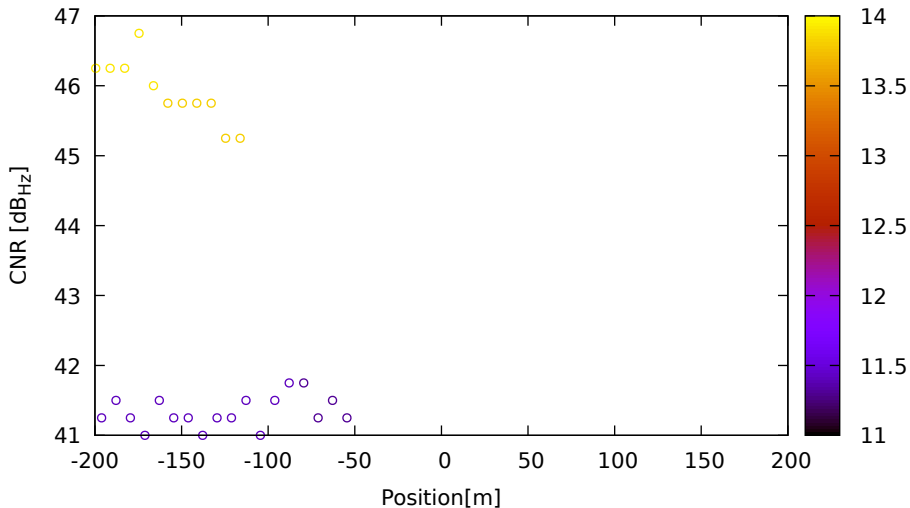
CNR vs position for G08 (L5) on LeicaGS15 - DOY 262 jam. 2
