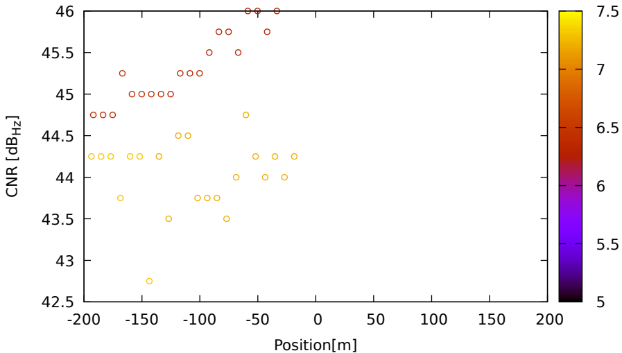
CNR vs position for G08 (L5) on LeicaGS15 - DOY 262 jam. 3
