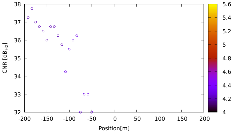
CNR vs position for G09 (L1) on LeicaGS15 - DOY 262 jam. 3
