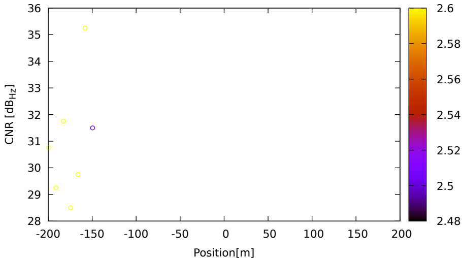
CNR vs position for G14 (L2) on LeicaGS15 - DOY 262 jam. 2
