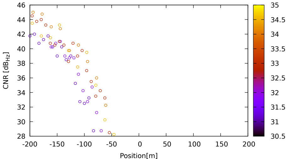
CNR vs position for G17 (L1) on LeicaGS15 - DOY 262 jam. 1
