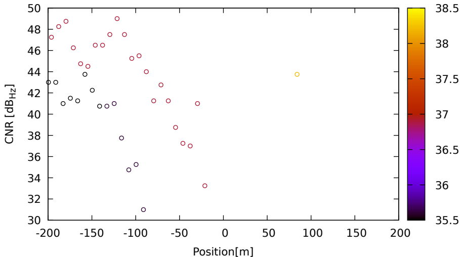
CNR vs position for G17 (L1) on LeicaGS15 - DOY 262 jam. 2
