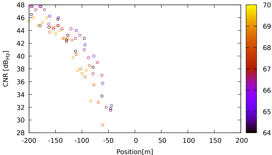
CNR vs position for G21 (L1) on LeicaGS15 - DOY 262 jam. 1
