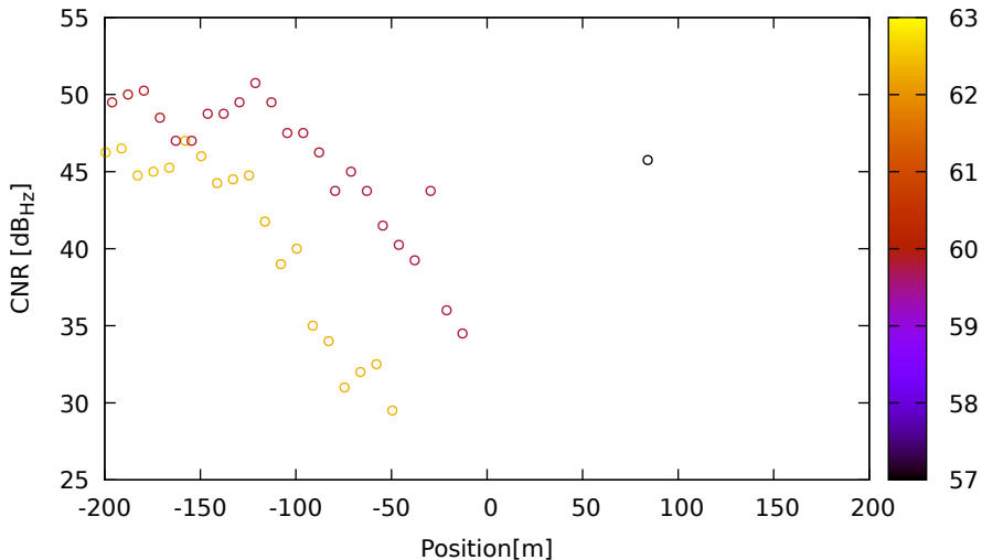
CNR vs position for G21 (L1) on LeicaGS15 - DOY 262 jam. 2
