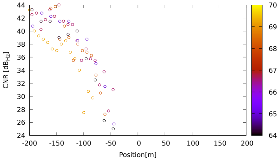
CNR vs position for G21 (L2) on LeicaGS15 - DOY 262 jam. 1
