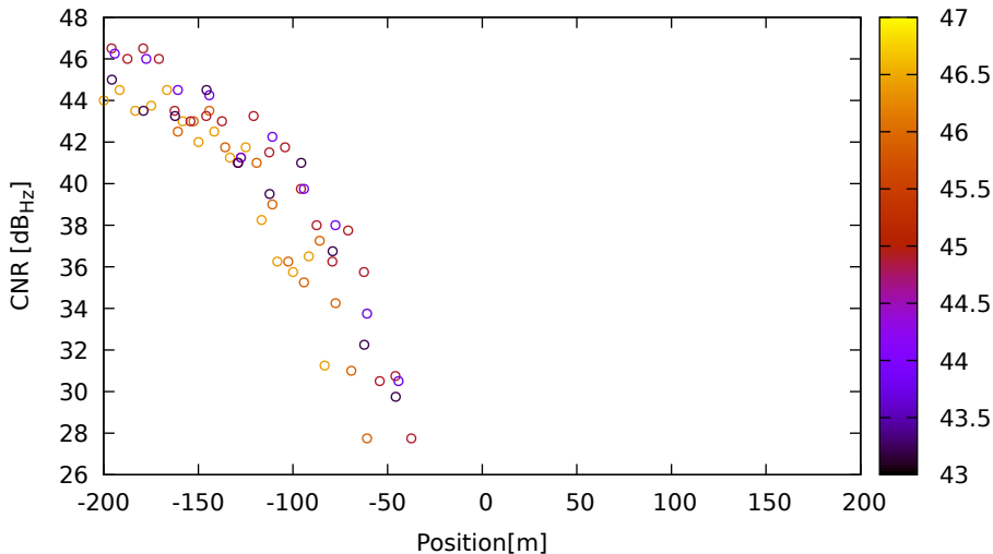
CNR vs position for G22 (L1) on LeicaGS15 - DOY 262 jam. 1
