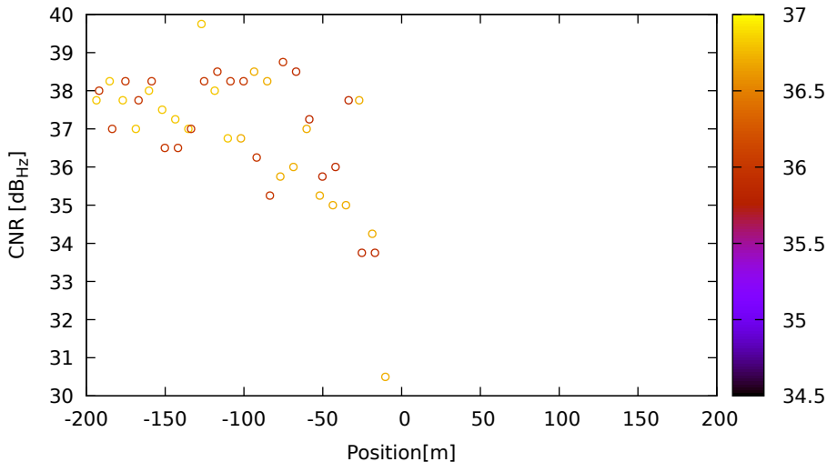
CNR vs position for G22 (L2) on LeicaGS15 - DOY 262 jam. 3
