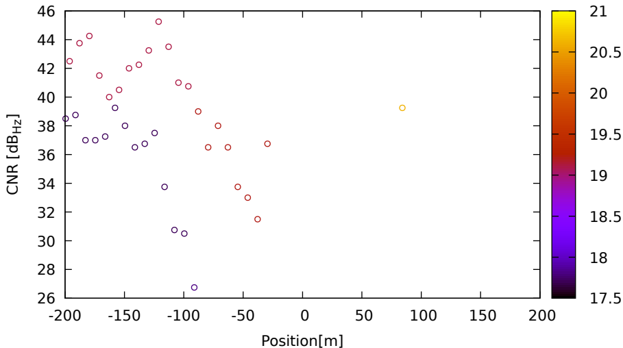
CNR vs position for G31 (L1) on LeicaGS15 - DOY 262 jam. 2
