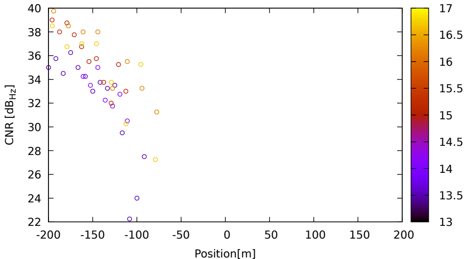
CNR vs position for G31 (L2) on LeicaGS15 - DOY 262 jam. 1
