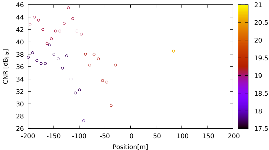
CNR vs position for G31 (L2) on LeicaGS15 - DOY 262 jam. 2
