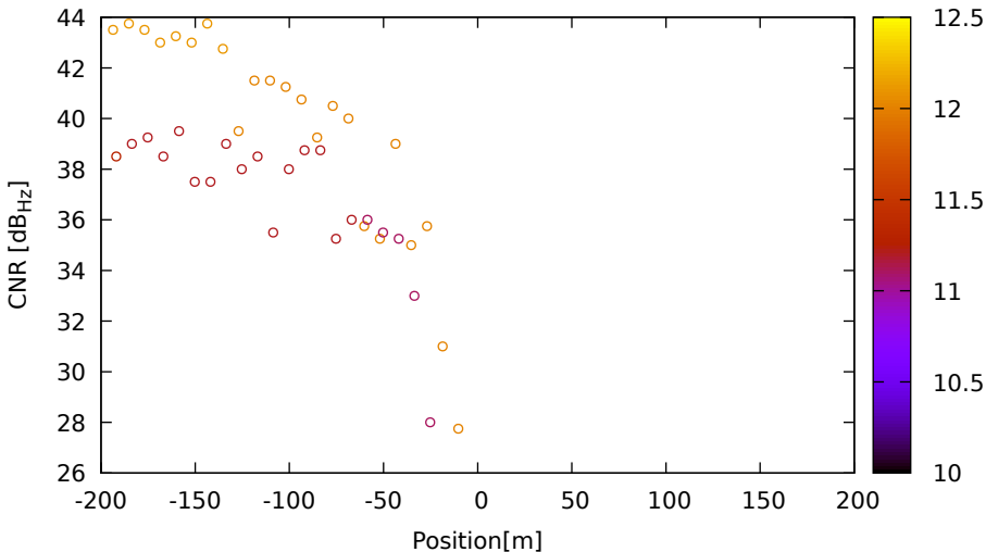
CNR vs position for G32 (L2) on LeicaGS15 - DOY 262 jam. 3
