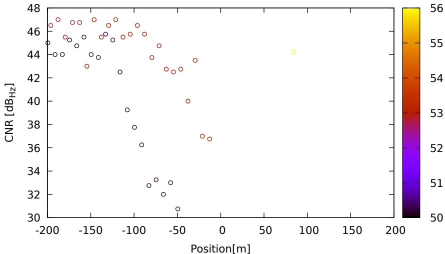
CNR vs position for R01 (G1) on LeicaGS15 - DOY 262 jam. 2
