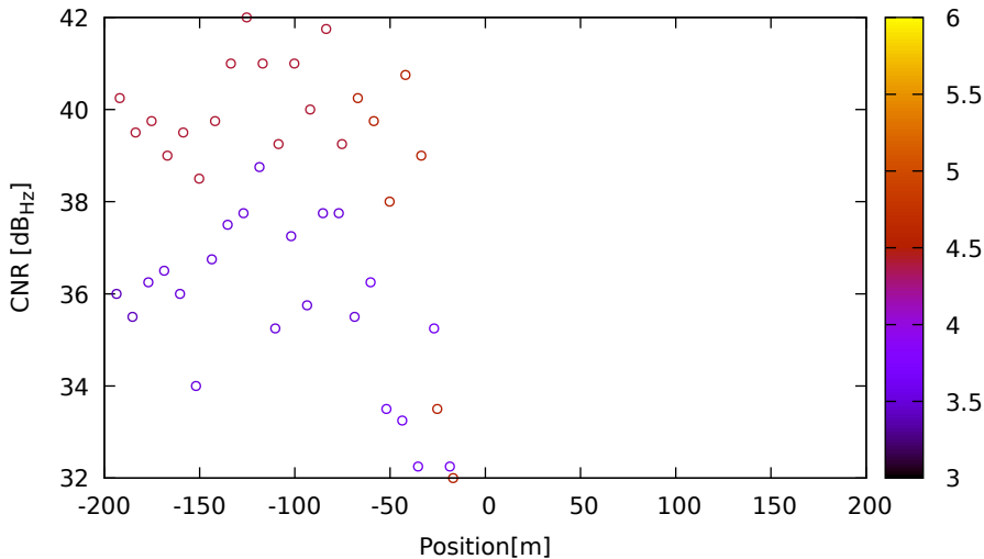
CNR vs position for R02 (G1) on LeicaGS15 - DOY 262 jam. 3
