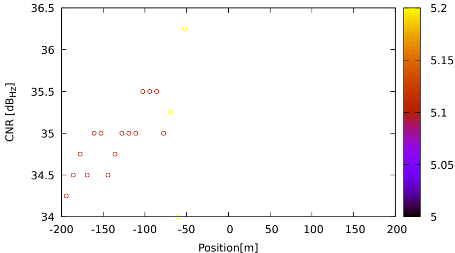
CNR vs position for R02 (G2) on LeicaGS15 - DOY 262 jam. 3
