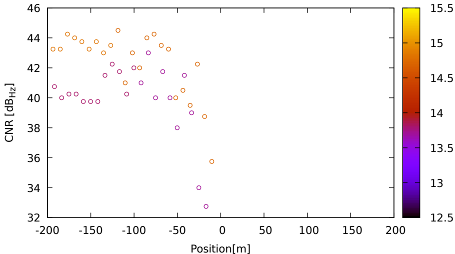
CNR vs position for R07 (G1) on LeicaGS15 - DOY 262 jam. 3
