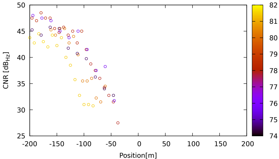
CNR vs position for R08 (G1) on LeicaGS15 - DOY 262 jam. 1
