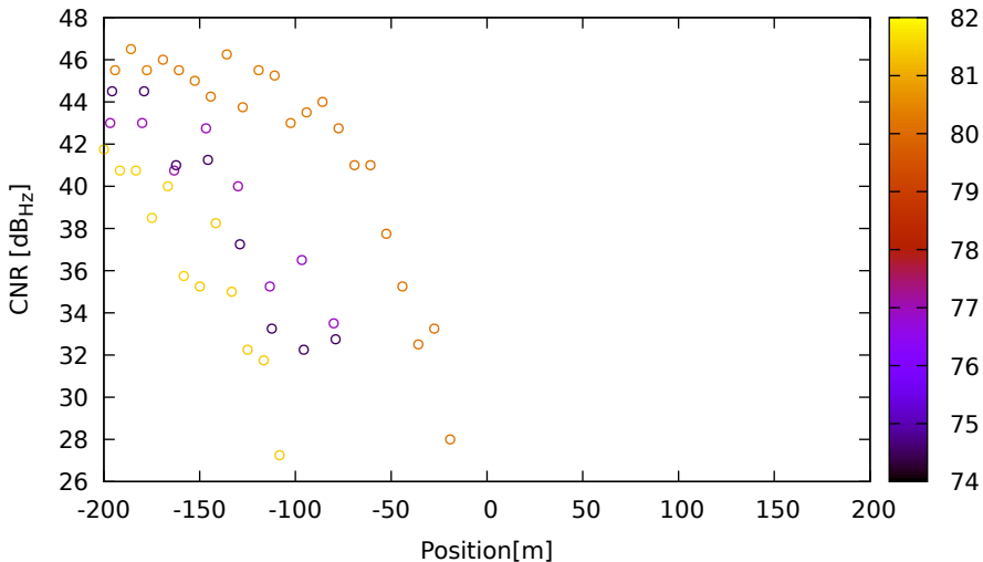
CNR vs position for R08 (G2) on LeicaGS15 - DOY 262 jam. 1
