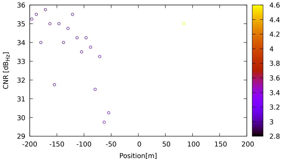
CNR vs position for R09 (G1) on LeicaGS15 - DOY 262 jam. 2
