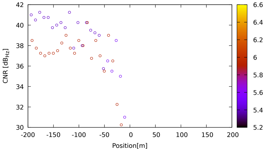
CNR vs position for R09 (G1) on LeicaGS15 - DOY 262 jam. 3
