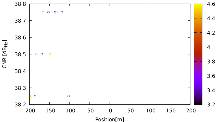
CNR vs position for R09 (G2) on LeicaGS15 - DOY 262 jam. 2
