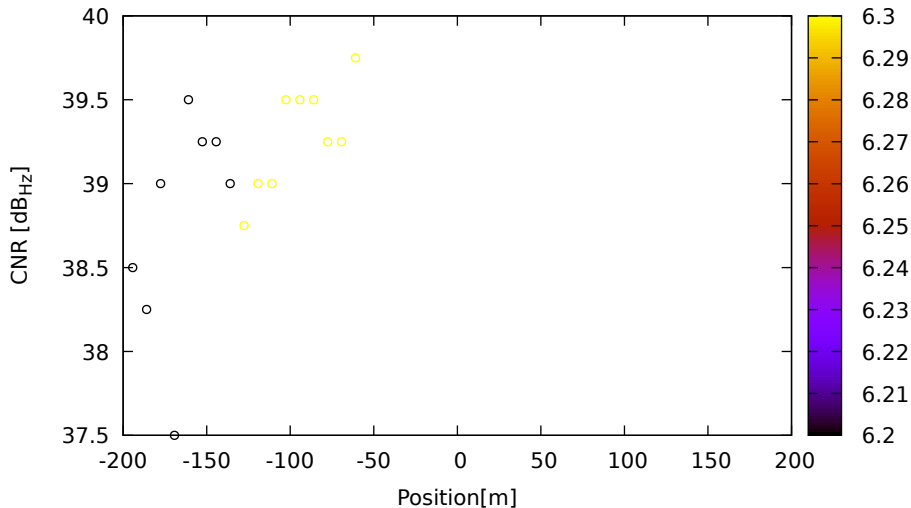
CNR vs position for R09 (G2) on LeicaGS15 - DOY 262 jam. 3
