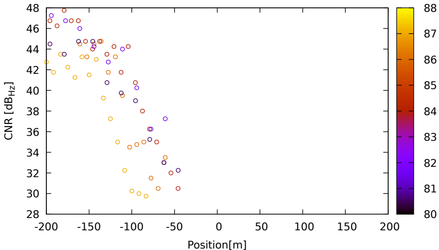
CNR vs position for R23 (G1) on LeicaGS15 - DOY 262 jam. 1
