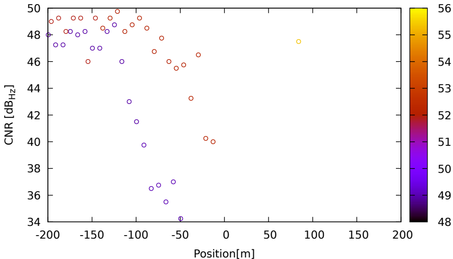
CNR vs position for R24 (G1) on LeicaGS15 - DOY 262 jam. 2
