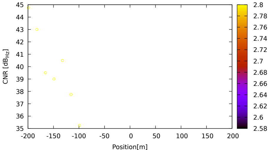
CNR vs position for E03 (E1) on LeicaGS15 - DOY 262 jam. 2
