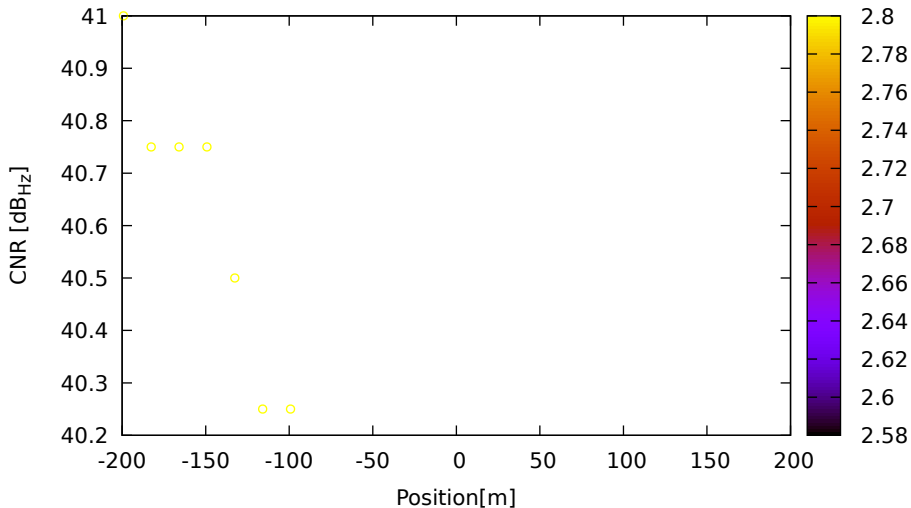
CNR vs position for E03 (E5) on LeicaGS15 - DOY 262 jam. 2
