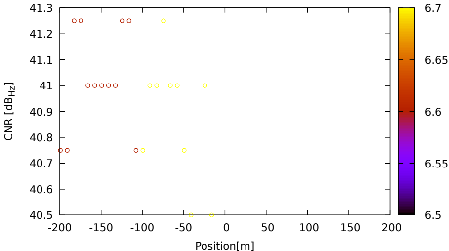
CNR vs position for E03 (E5a) on LeicaGS15 - DOY 262 jam. 3
