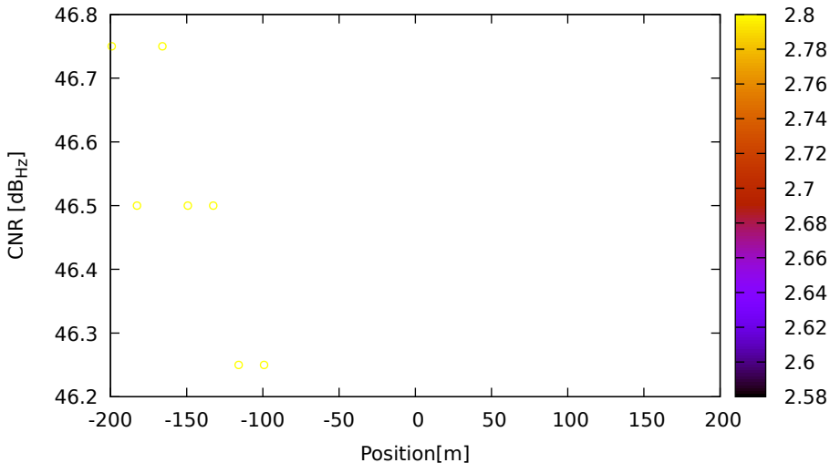
CNR vs position for E03 (E5b) on LeicaGS15 - DOY 262 jam. 2
