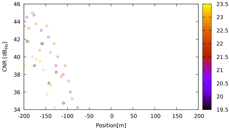
CNR vs position for E04 (E1) on LeicaGS15 - DOY 262 jam. 1
