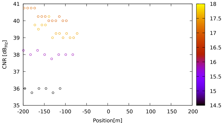
CNR vs position for E04 (E5) on LeicaGS15 - DOY 262 jam. 2
