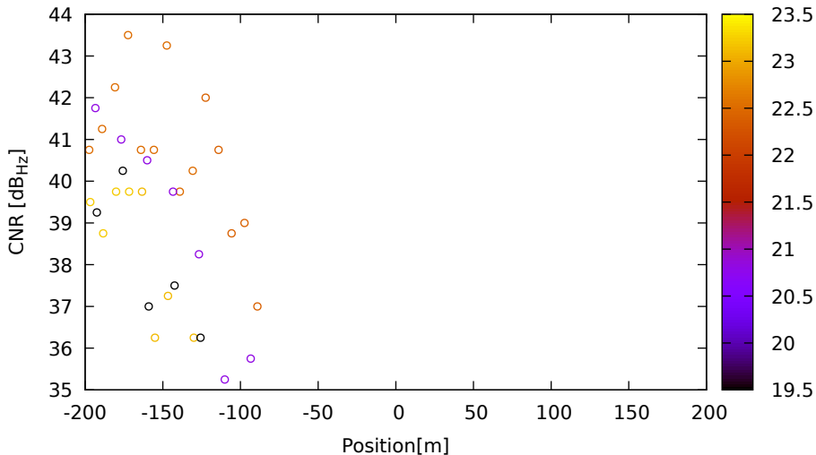
CNR vs position for E04 (E5a) on LeicaGS15 - DOY 262 jam. 1
