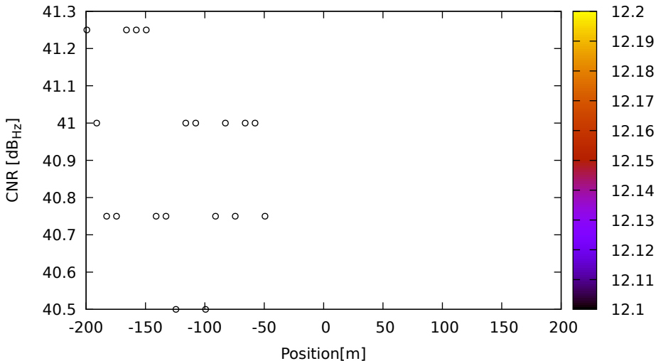
CNR vs position for E04 (E5a) on LeicaGS15 - DOY 262 jam. 3
