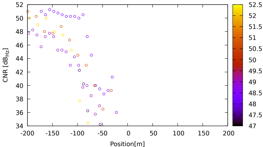
CNR vs position for E05 (E1) on LeicaGS15 - DOY 262 jam. 2
