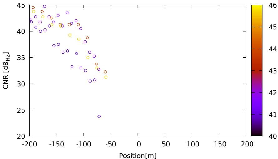
CNR vs position for E05 (E5) on LeicaGS15 - DOY 262 jam. 1
